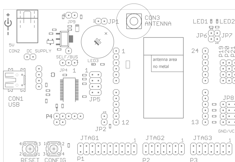
Figure 11: Assembly diagram
