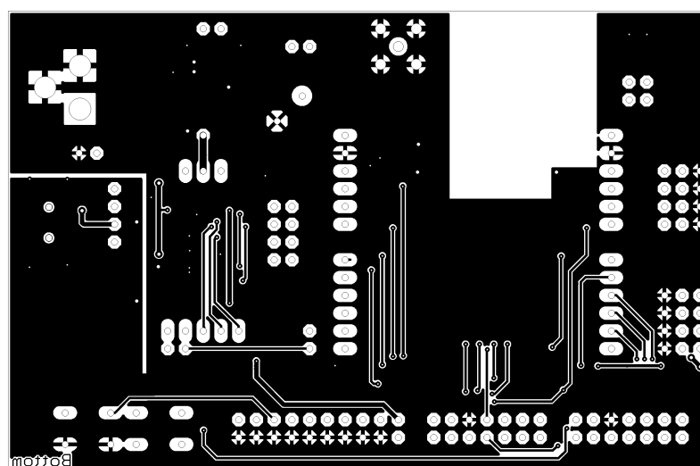
Figure 12: Top and Bottom Layer
