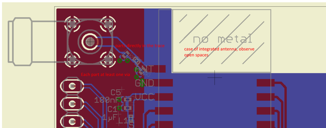
Figure 5: Layout
