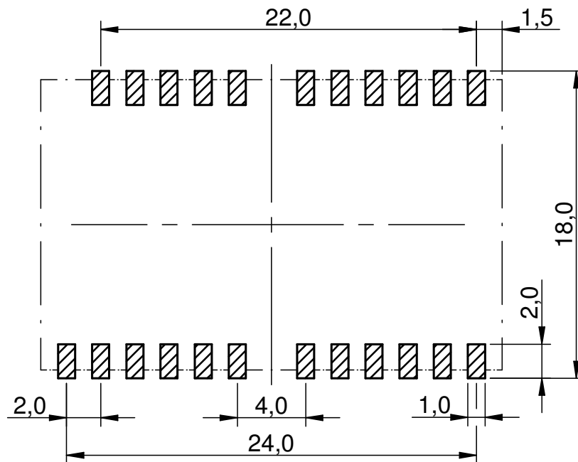
Figure 15: Footprint and dimensions [mm]
