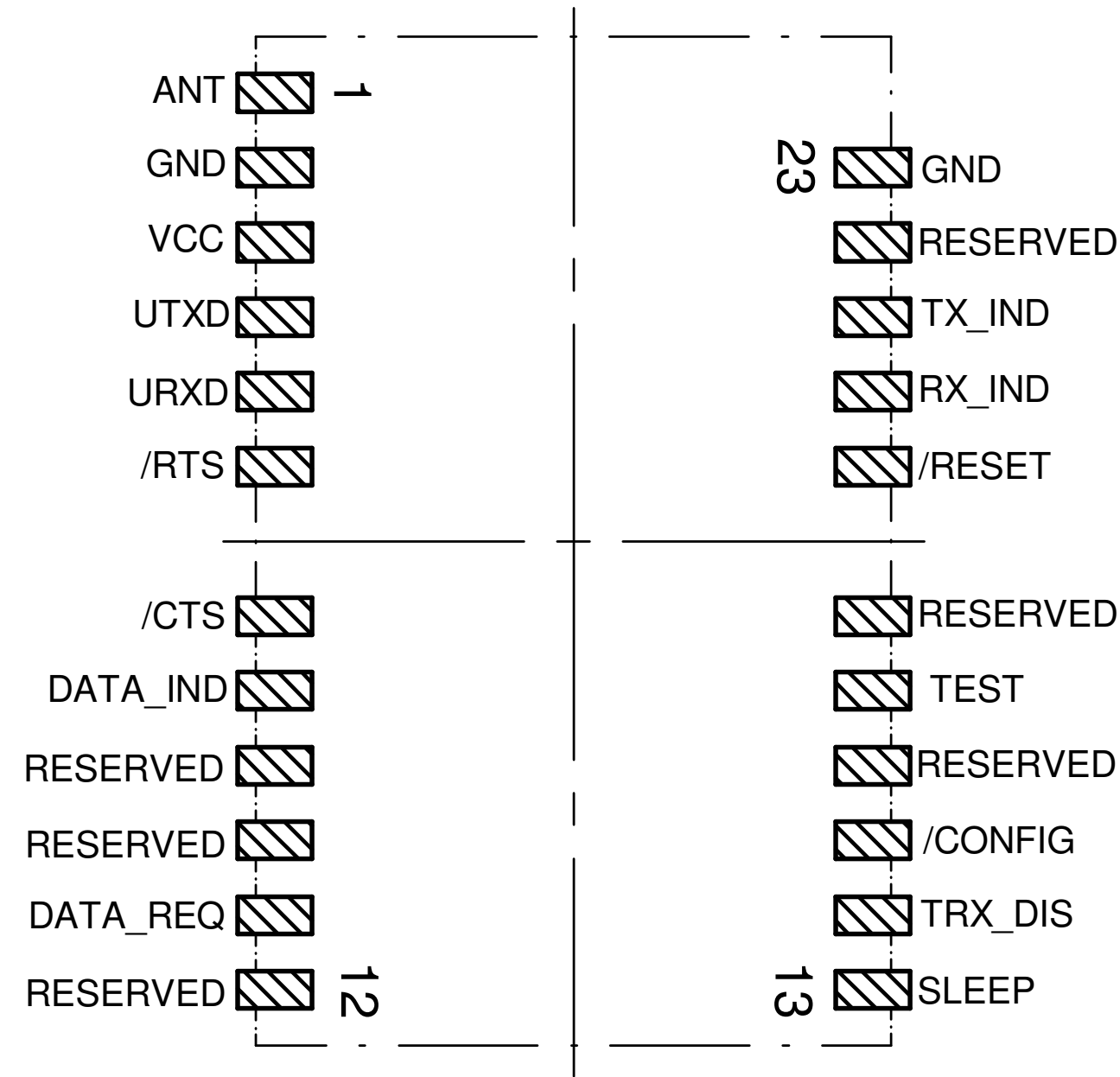
Figure 2: Pinout
